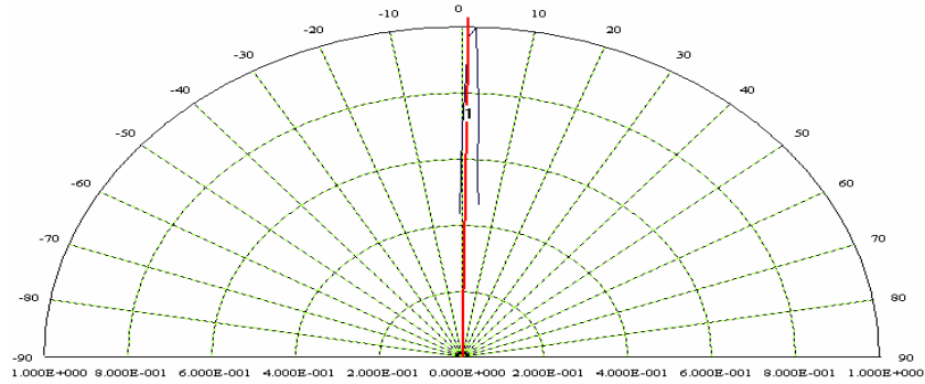
Typical Angular Diagram UVTOPxxxTO39BL
