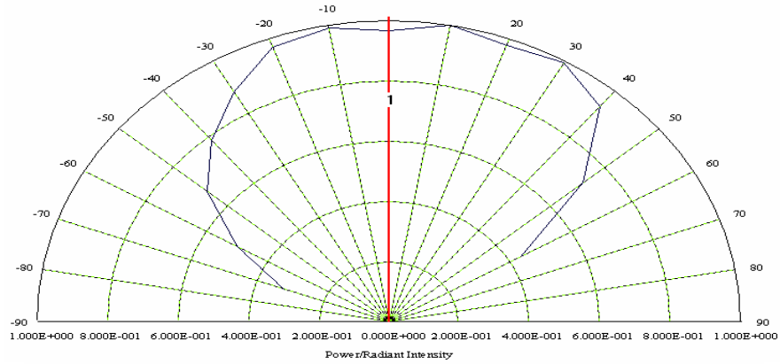
Typical Angular Diagram UVTOPxxxTO39HS
