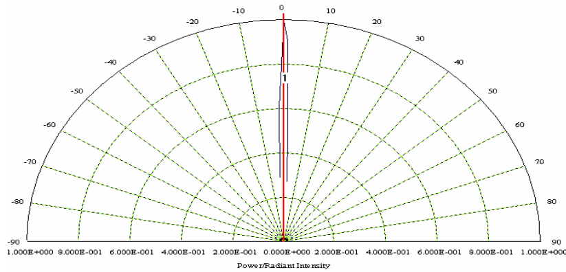
Typical Angular Diagram UVTOPxxxTO39BL
