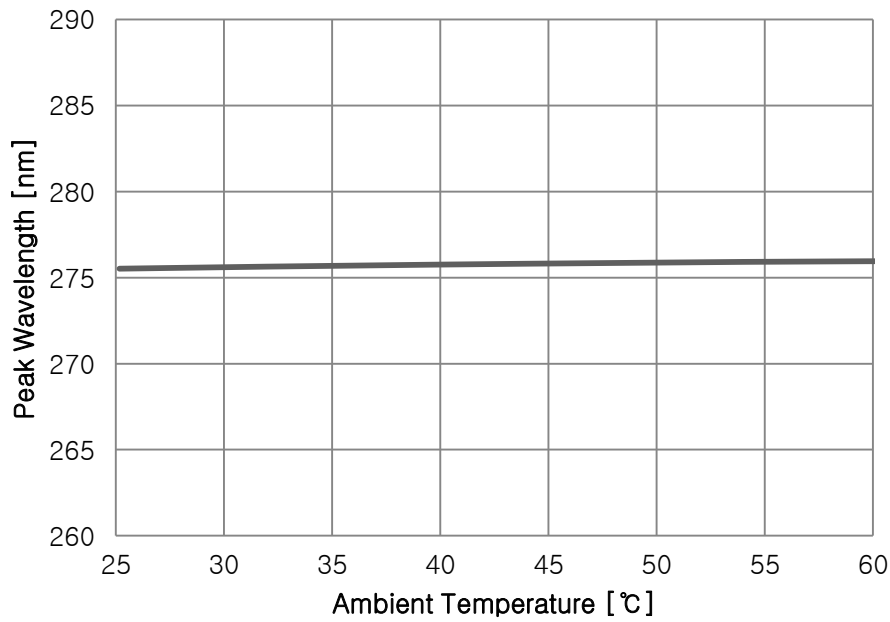
Fig 6. Peak Wavelength vs. Ambient Temperature, I_F=20\text{mA}
