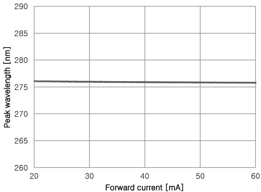
Fig 4. Peak Wavelength vs. Forward Current, T_a=25^\circ\text{C}
