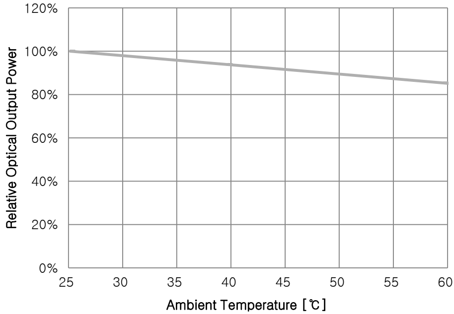
Fig 5. Relative Optical Output Power vs. Ambient Temperature, I_F=20\text{mA}
